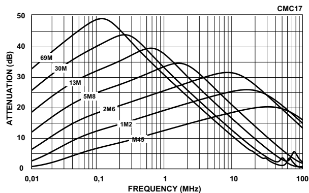
Typical values (Z=50Ω) at 25°C with 1mT at 10kHz
